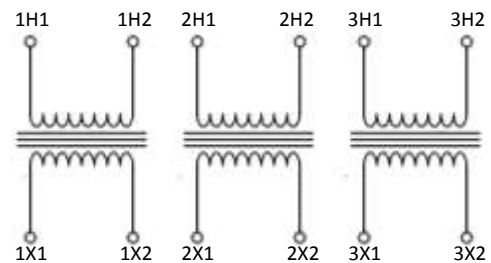
CONNECTION DIAGRAM
