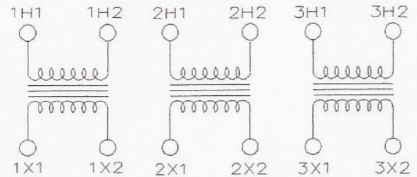
CONNECTION DIAGRAM
